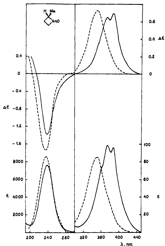
Figure 2. CD and UV spectra of N -nitrosoazetidine 2 in heptane (—) and MeOH (---).
