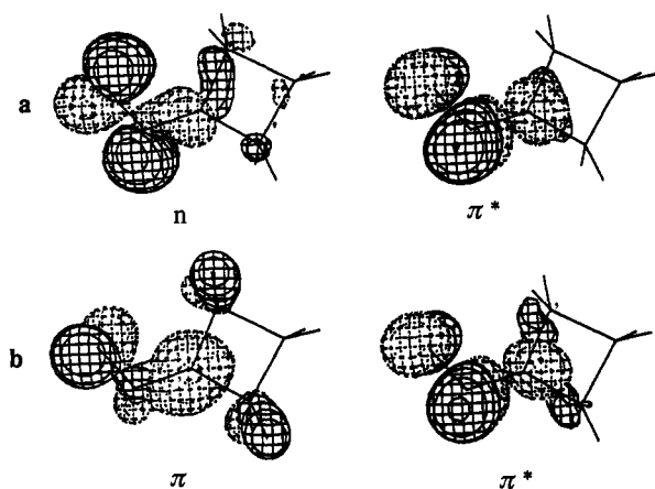
Figure 4. Singly occupied molecular orbitals of the two lowest excited states of 1-nitrosoazetidine (1): (a) first excited state ( n-\pi^* ). (b) second excited state ( \pi-\pi^* ).
