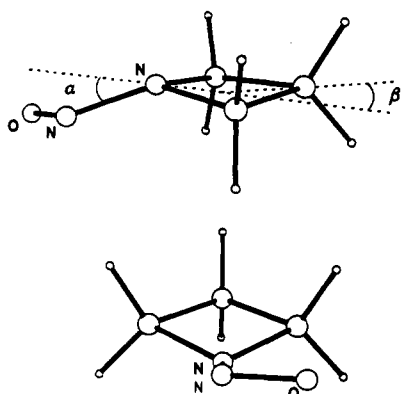
Figure 1. 6-31G* structure of the -sc rotamer of 1-nitrosoazetidines (1) (see Table 1).
